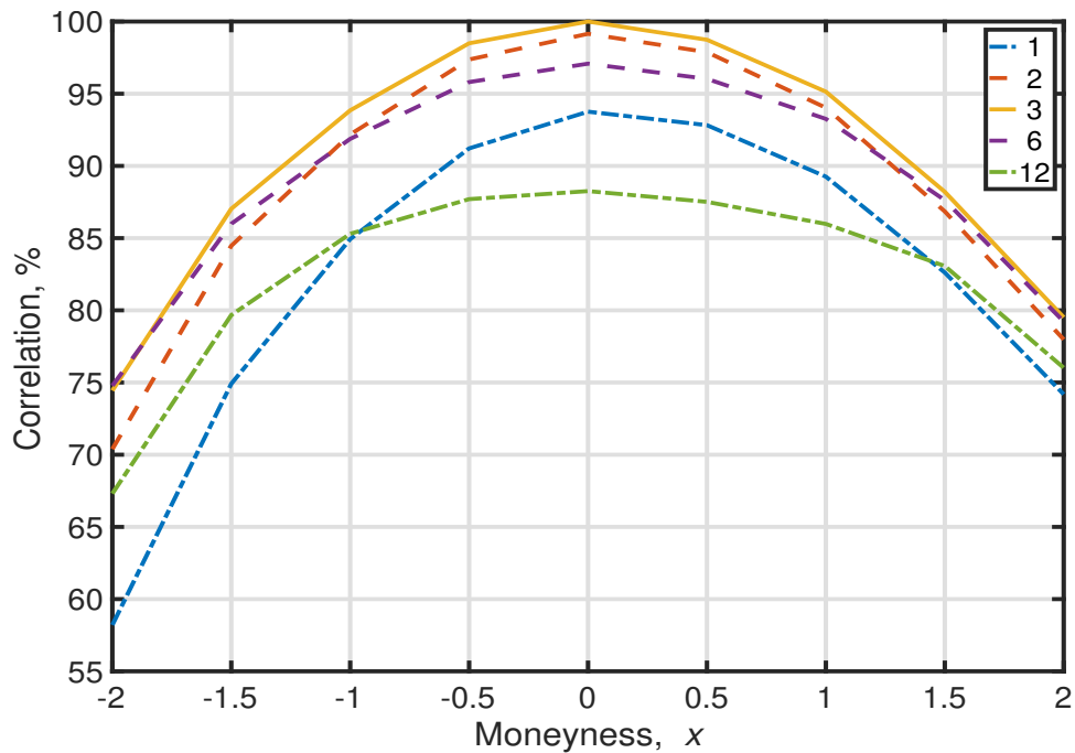
Figure 1. Implied volatility change correlation with the three-month at-the-money option. The plots show the cross-correlation estimates of percentage implied volatility changes between the reference three-month at-the-money option contract and contracts at other maturities and moneyness. Each line represents the correlation variation across moneyness at one maturity. The solid line denotes the correlation estimates with contracts at the same three-month maturity. The two dashed lines denote estimates with contracts at the two adjacent maturities at two and six months. The two dash-dotted lines denote estimates with contracts at further apart maturities at one and 12 months.
