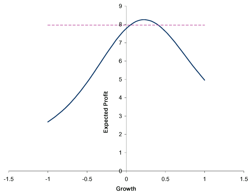
Figure 4: Expected profit, hedging using implied volatility, versus growth rate \mu ; S = 100, \sigma = 0.4, r = 0.05, D = 0, E = 110, T = 1, \tilde{\sigma} = 0.2 . The dashed line is the profit to be made when hedging with actual volatility.
