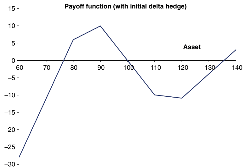
Figure 19: Payoff with initial delta hedge for optimal portfolio; S = 100 , \mu = 0 , \sigma = 0.2 , r = 0.05 , D = 0 , T = 1 . See text for additional parameters and information.
