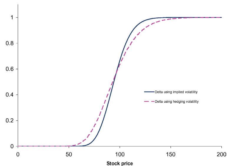
Figure 16: Deltas based on implied volatility and hedging volatility. E = 100 , S = 100 , r = 0.1 , D = 0 , T = 0.5 , \tilde{\sigma} = 0.2 , \sigma^h = 0.3 .
