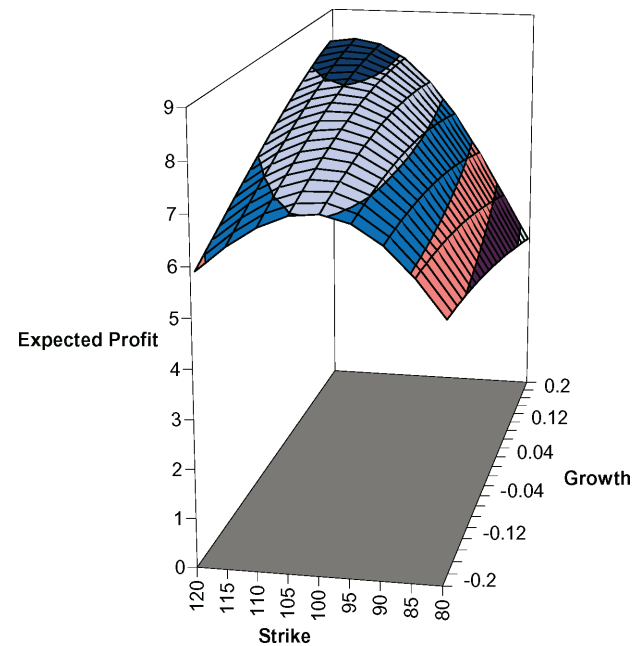
Figure 5: Expected profit, hedging using implied volatility, versus growth rate \mu and strike E ; S = 100, \sigma = 0.4, r = 0.05, D = 0, T = 1, \tilde{\sigma} = 0.2 .
