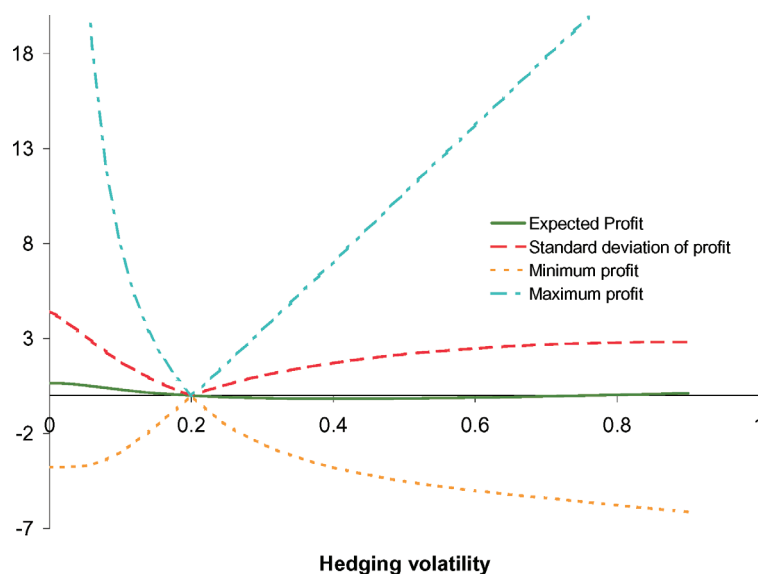
Figure 13: Expected profit, standard deviation of profit, minimum and maximum, hedging with various volatilities. E = 100, S = 100, \mu = 0, \sigma = 0.2, r = 0.1, D = 0, T = 1, \tilde{\sigma} = 0.2 .
