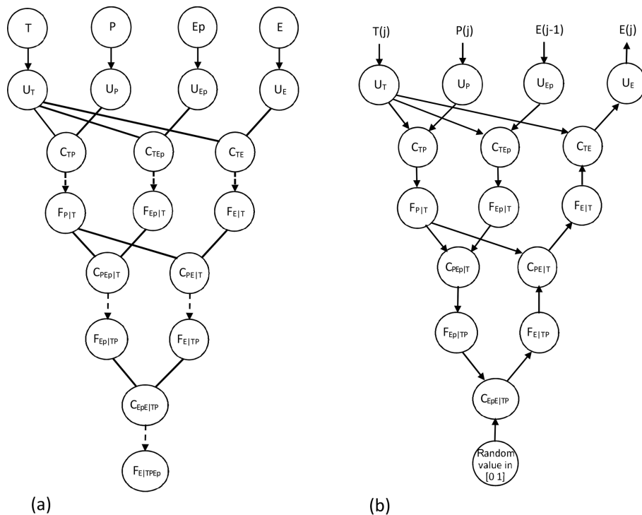
Figure 3. Construction of C-vine copula V_{TPE_pE} (a) and simulation of E from V_{TPE_pE} (b).
