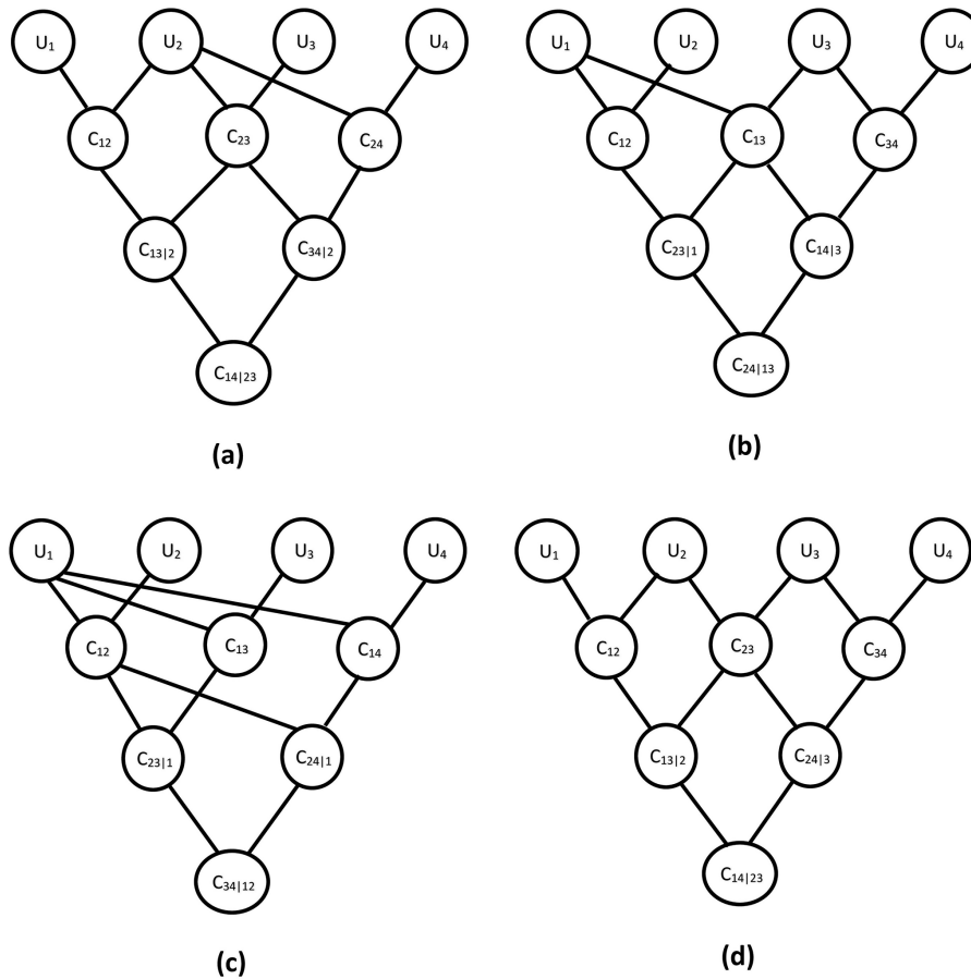
Figure 2. Examples of four-dimensional vine copulas: (a, b) regular vine copulas, (c) canonical vine or C-vine copula and (d) D-vine copula.
