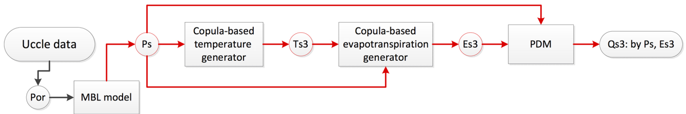
Figure 11. Different cases for discharge simulation. P_{Or} , E_{Or} and T_{Or} refer to the observed time series. P_s , E_{s1} , E_{s2} , E_{s3} , T_{s2} and T_{s3} refer to the simulated time series (red blocks). Red arrows indicate the simulation processes related to stochastically generated time series.
