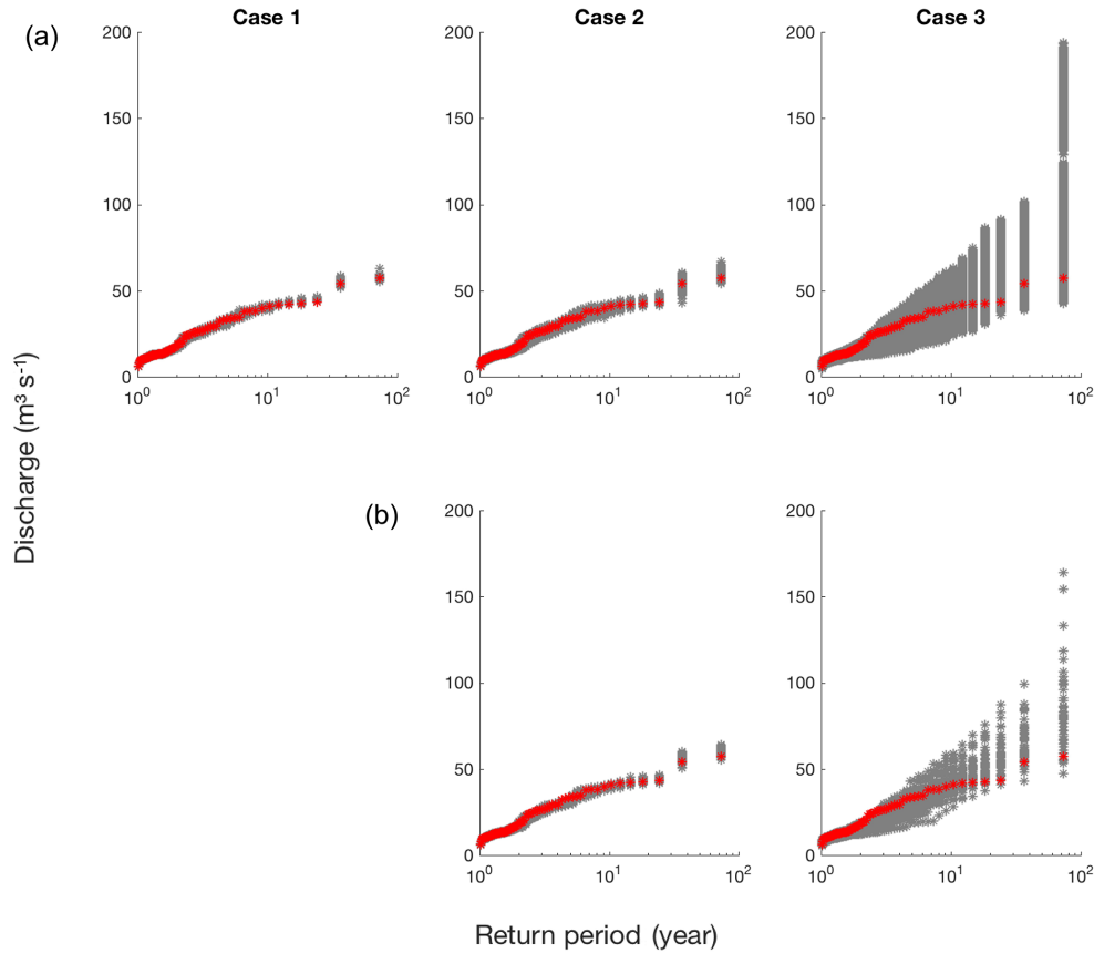
Figure 15. Comparison between the empirical return periods of annual extremes of the observed and simulated discharge for all cases. Reference discharge Q_{rf} is in red and the ensemble of time series of simulated discharge is in grey. The top row shows extremes obtained on the basis of unequal ensemble widths of 50 (case 1), 2500 (case 2) or 125 000 (case 3) time series. The bottom row shows extremes obtained on the basis of equal ensemble widths of 50 time series.
