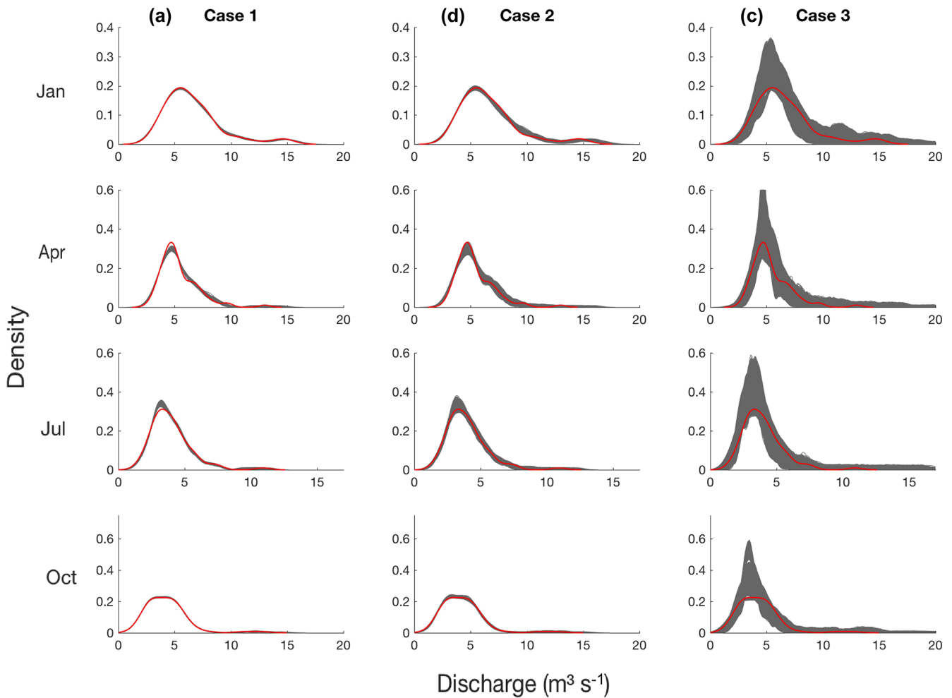
Figure 17. Comparison between the probability density functions of the mean of discharge of the observed and simulated values in three cases. Reference discharge Q_{rf} is in red and the time series of simulated discharge is in grey.
