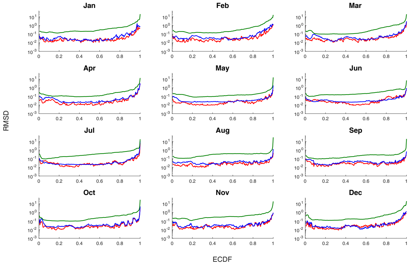
Figure 18. Root mean square difference (RMSD) for simulated discharge in different cases: case 1 (red), case 2 (blue) and case 3 (green). The RMSD is plotted against the cumulative relative frequency of the discharge given by the empirical cumulative distribution (ECDF) value.
