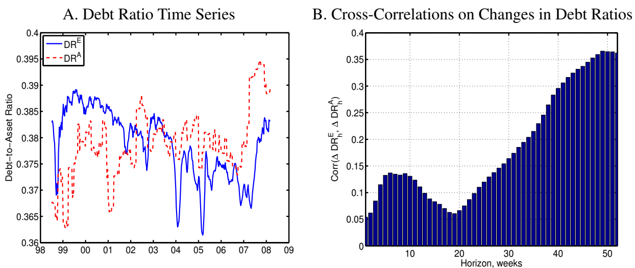
Figure 3. Debt-to-asset ratios extracted from equity index options and accounting reports. Panel A plots the time series of two debt-to-asset ratios, with the solid line denoting the series extracted from equity index options ( DR^E ) based on our model specification and parameter estimates and the dashed line denoting the corresponding estimates compiled from accounting reports ( DR^A ). The lines are scaled to have the same sample mean and standard deviation. The bars in panel B represent the cross-correlation estimates between changes in the two sets of debt ratios over different horizons.
