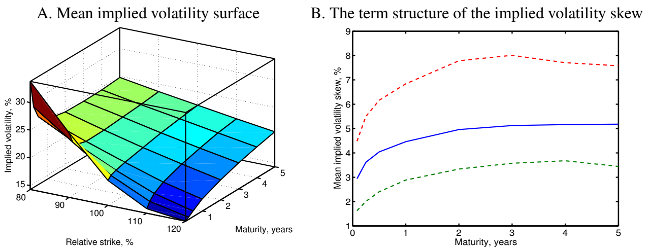
Figure 4. The mean implied volatility surface and implied volatility skew.
